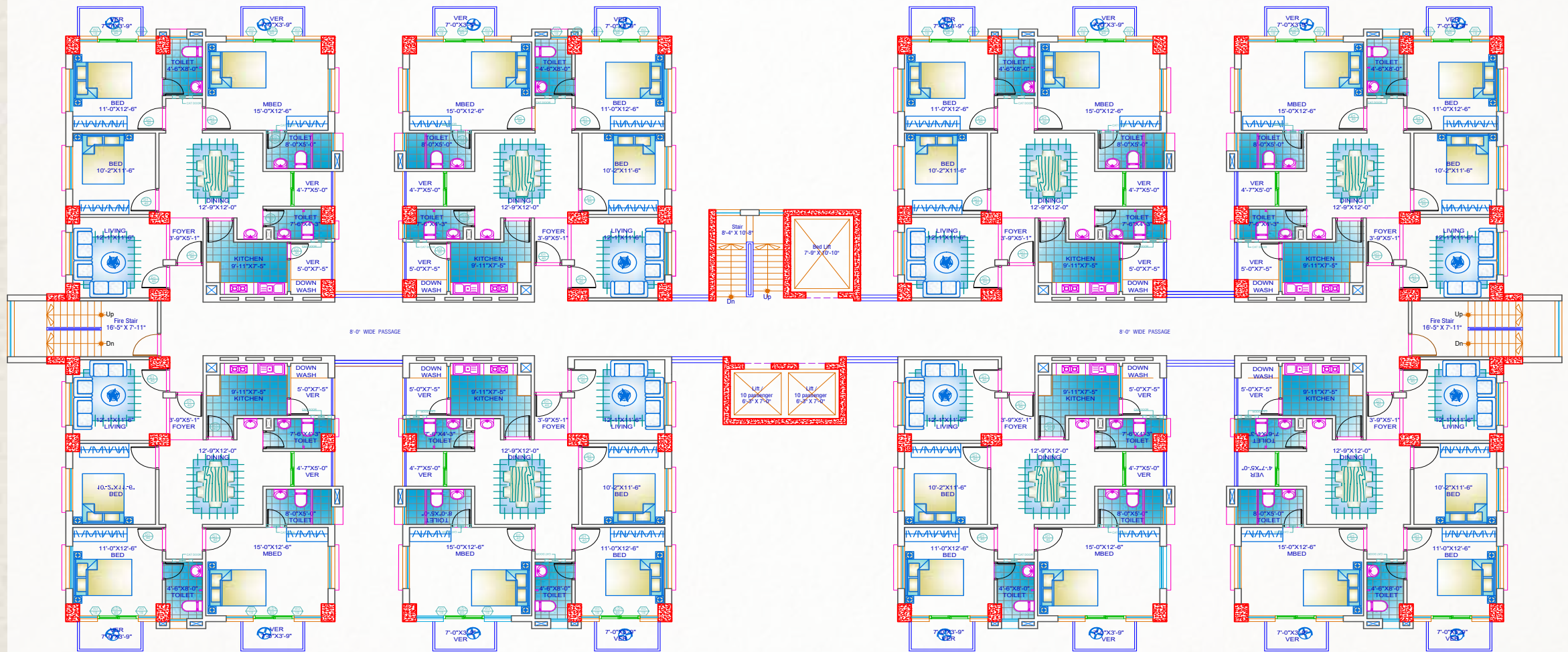
Typical Floor Plan
